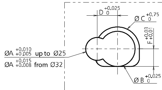
POCKET DIMENSIONS
